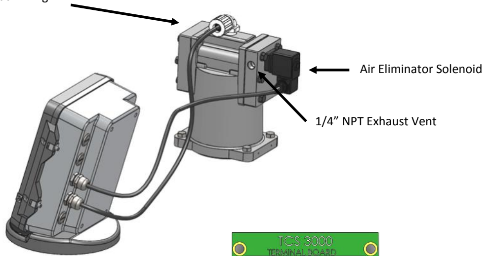
Air Eliminator Float Wiring
