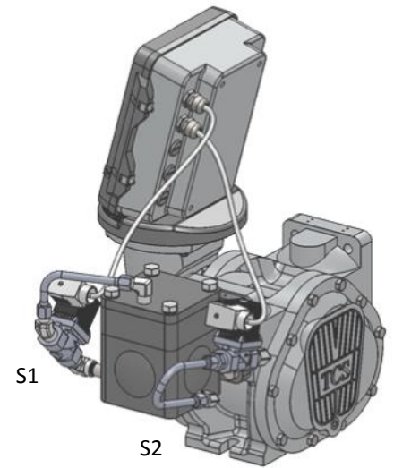
755-31 Diaphragm 3" Valve
