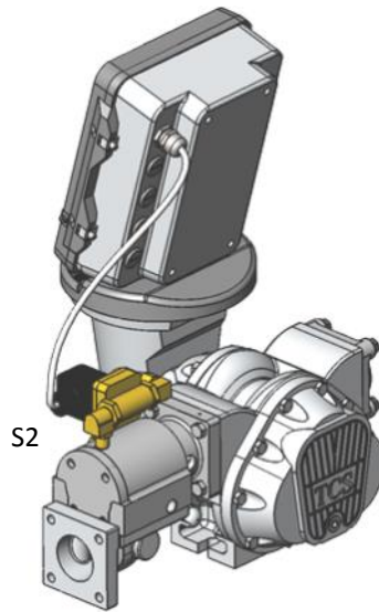
755-21 Piston 2" Valve
