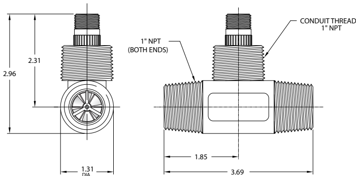
Figure 3: Dimensions
