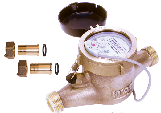
MJN-Series (brass body)
